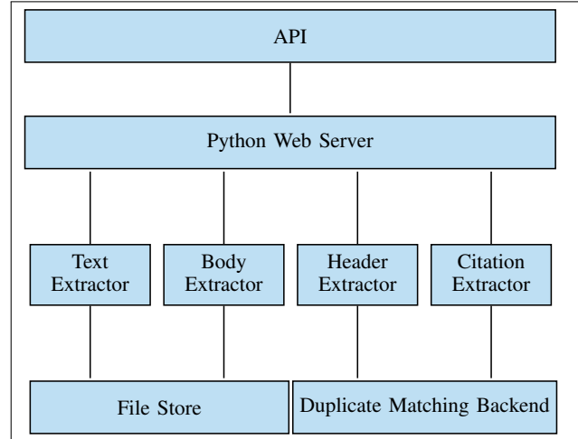
Figure 2. CiteSeerExtractor architecture
