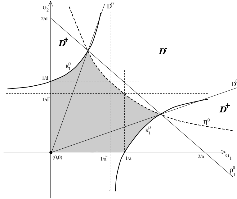
Figure 3: An illustration for the proof of Theorem 2. a, d > 0 , bc < 0 . All (G_1, G_2) \in \mathcal{D}^- and below the right branch of \eta^0 (dashed line) correspond to the attractive fixed points. So do (G_1, G_2) \in (0, 1/4]^2 in \mathcal{D}^+ between the two branches of \kappa_1^0 .
