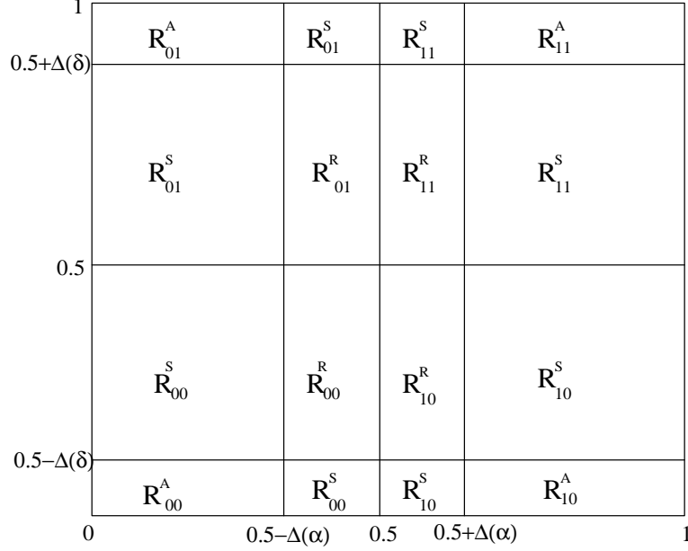
Figure 5: Partitioning of the network state space according to stability types of the fixed points.
