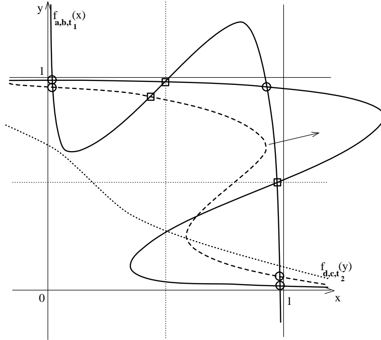
Figure 9: Geometrical illustration of saddle-node bifurcation in a recurrent neural network with two state neurons. Saddle and attractive points are marked with squares and circles respectively. a, d > 0 , b, c < 0 .
