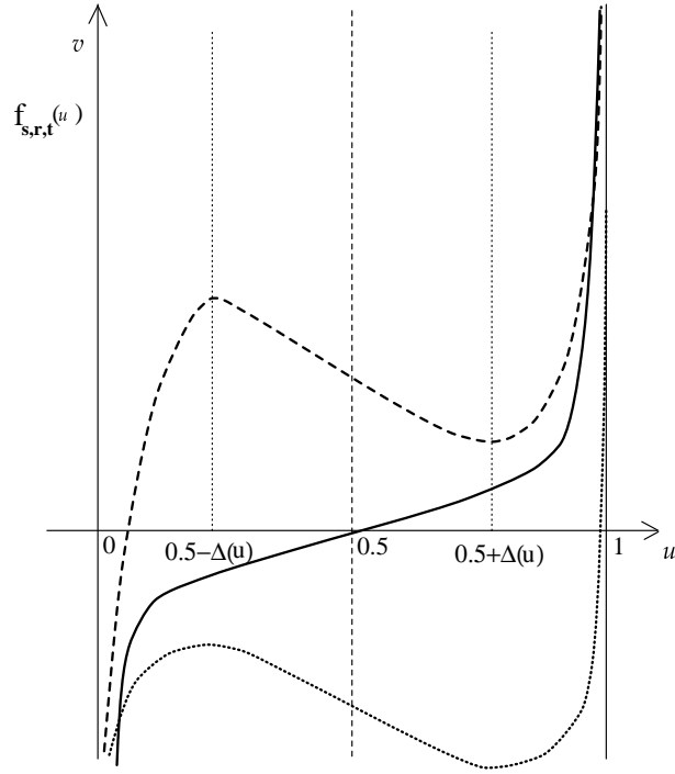
Figure 6: Graph of f_{s,r,t}(u) . Solid and dotted lines represent the cases t, s = 0, r > 0 and t = 0, s > 4, r > 0 . Dashed line shows the graph when t < 0, s > 4 and r > 0 . Negative external input t shifts the bended part into v > 0 .
