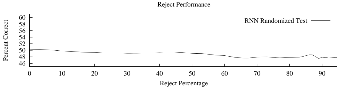
Figure 9. Classification performance as the confidence threshold is increased for the randomized test sets. This graph is the average of the individual randomized test sets.
