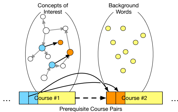
Figure 2: Process of synthetic data generation. After a concept prerequisite graph is created, prerequisite course pairs are generated by blending prerequisite concept pairs with background words.
