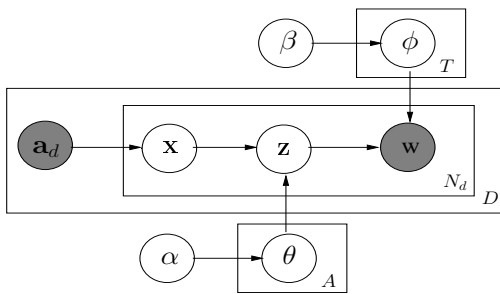
(b) The author-topic model [20].
