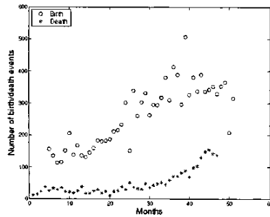
(a) Node
