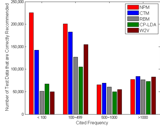
Figure 4: Performance versus papers’ cited frequency.
