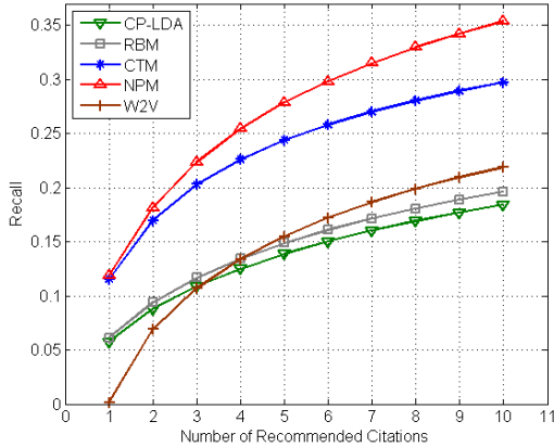
Figure 3: Recall as the number of recommended citations ranges from 1 to 10.
