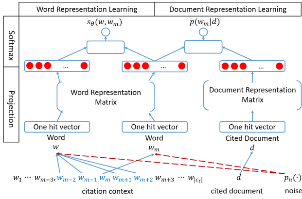
Figure 2: Neural network architecture for word and document representation learning.
